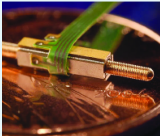
Smaller and smaller piezoelectric motors, such as this SQUIGGLE motor from New Scale, are opening up new applications in consumer electronic devices.
